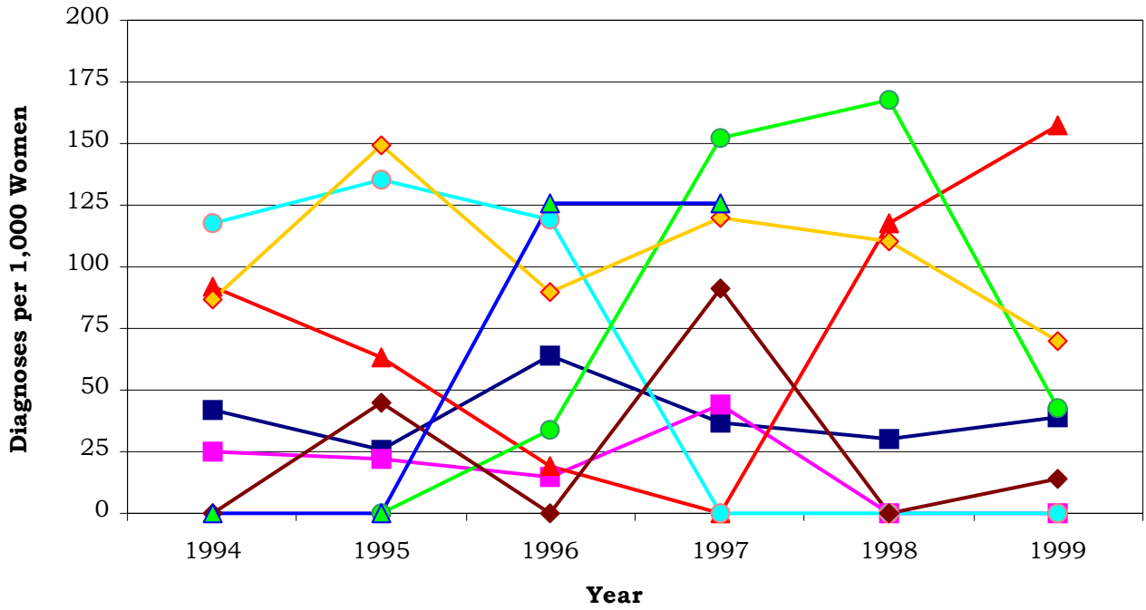
Figure 19. Age-Adjusted Rates for All OSHA-Recordable Diagnoses Combined Among Women and Men by Job Category from 1994 to 1999
