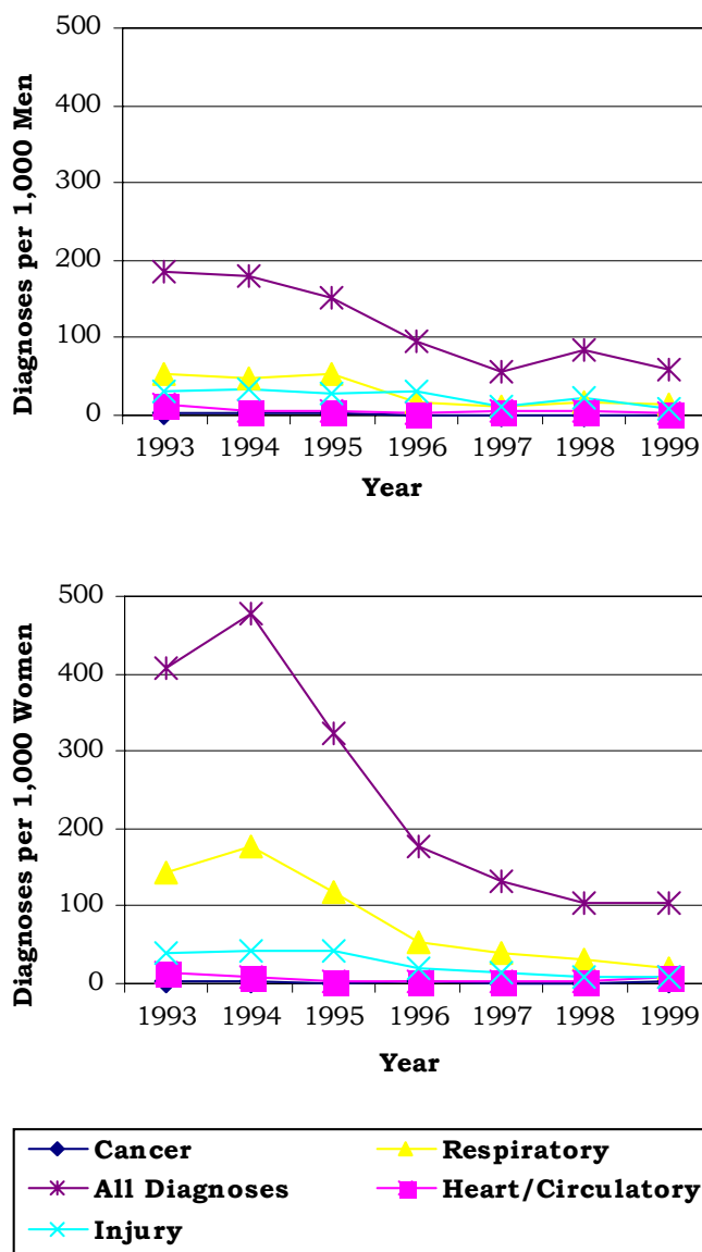
Figure 10. Age-Adjusted Rates for Selected Diagnostic Categories Among Men and Women from 1993 to 1999
