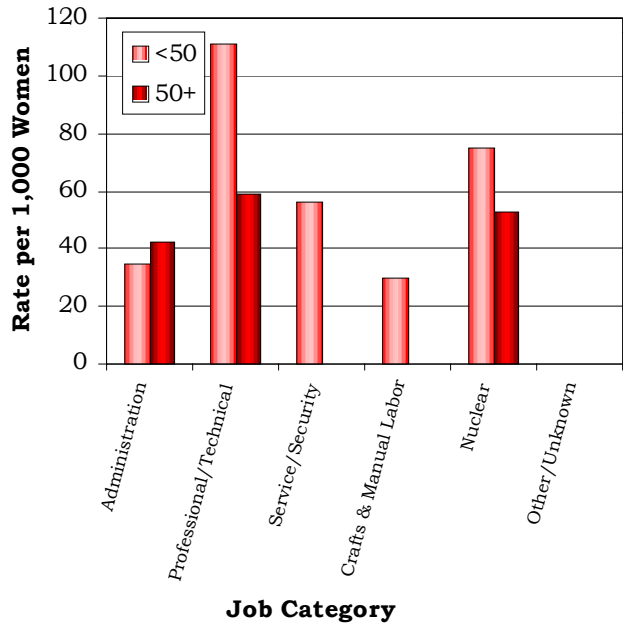
Figure 17. OSHA-Recordable Rates by Age and Job Categories Among Women, All Diagnoses Combined
