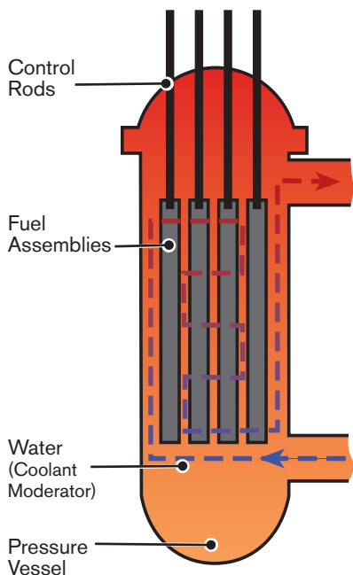
The fuel assemblies, control rods, and coolant make up the reactor's core. The core is surrounded by a massive steel pressure vessel.
